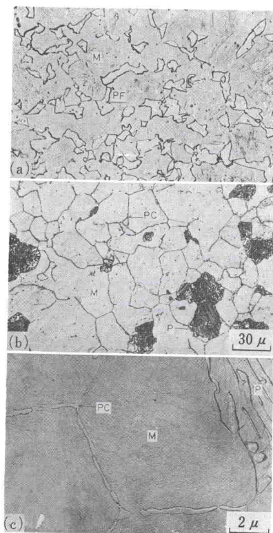
Photo. 3. Comparison of the transformation products formed in 0.49%C steel at 1 atm and 38.5 kbar (a) Proeutectoid ferrite (PF) in martensite matrix (M); 1 atm, 700°C×2 min (b), (c) Proeutectoid carbide (PC) and pearlite (P) in martensite matrix (M); 38.5 kbar, 650°C×1 hr
