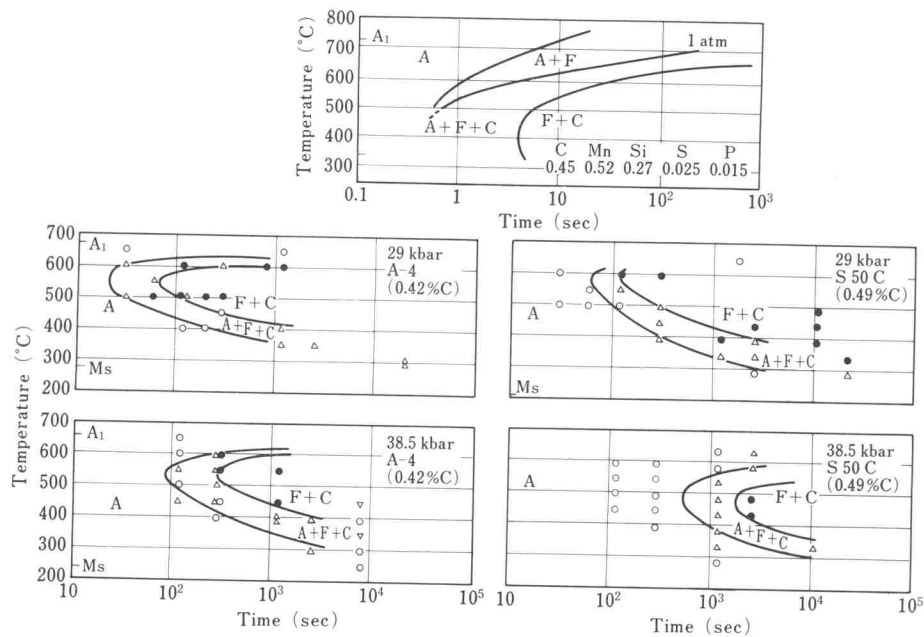
Fig. 3. TTT diagrams obtained in Fe-0.42%C alloy and 0.49%C commercial steel under high pressure. For comparison, a diagram 16) of 0.45%C steel at 1 atm is quoted at the top
